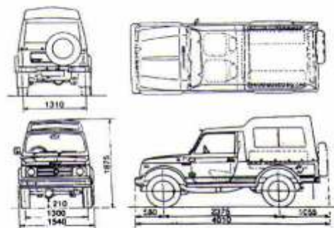
All Dimensions in mm. Shown Soft top version.
